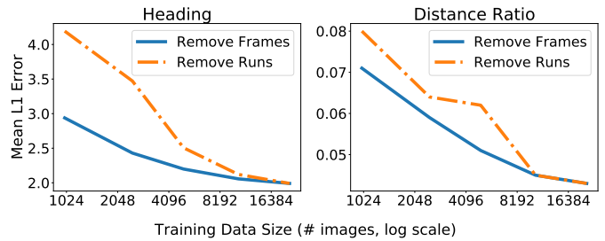
Fig. 10: Performance as a function of amount of training data. We sub-sample training data by either removing entire data collection runs, or by removing frames. Our perception model starts doing well even with small amounts of data.
